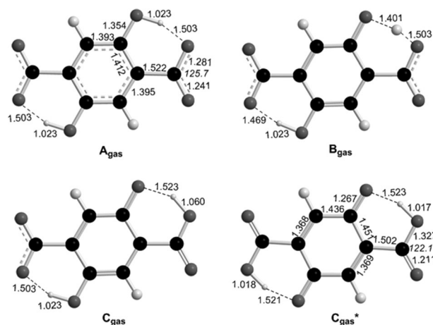
Figure 6. Selected structural parameters of minimum energy structures of H_2dhtp^{2-} located on the PESs in gas phase (C black, O gray, H light gray). A_{\text{gas}} , B_{\text{gas}} , C_{\text{gas}} , correspond to S_0 states of fluorophore structures located on the ESIPT PES and C_{\text{gas}}^* corresponds to the S_1 state of the lowest-energy fluorophore structure located on the ESIPT PES.
